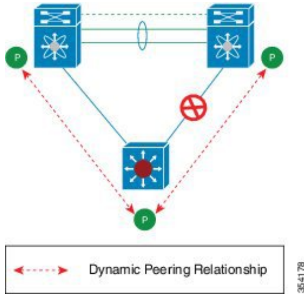
Figure 7: Supported: Peering Over an Orphan Device with Both the vPC Peers.
