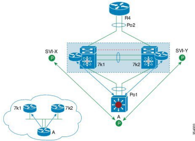
Figure 4: Layer 3 Over vPC Solution
