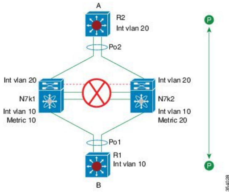
Figure 11: Unsupported: Peering Over vPC+ Interfaces in Cisco NX-OS 7.2(0)D1(1)
