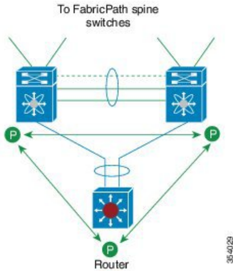
Figure 13: Unsupported: Route Peering with Orphan Device with Both the vPC+ Peers
