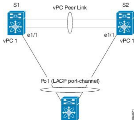
Figure 17: Physical Port vPC Topology
