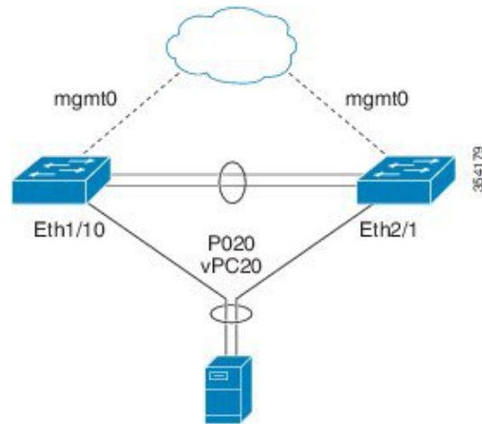
Figure 15: Switch vPC Topology
