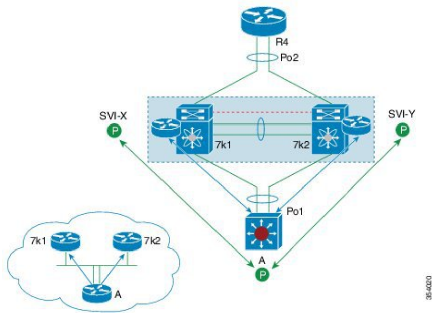
Figure 5: Supported: Peering Over a vPC Interconnection Where the Router Peers with Both the vPC Peers.
