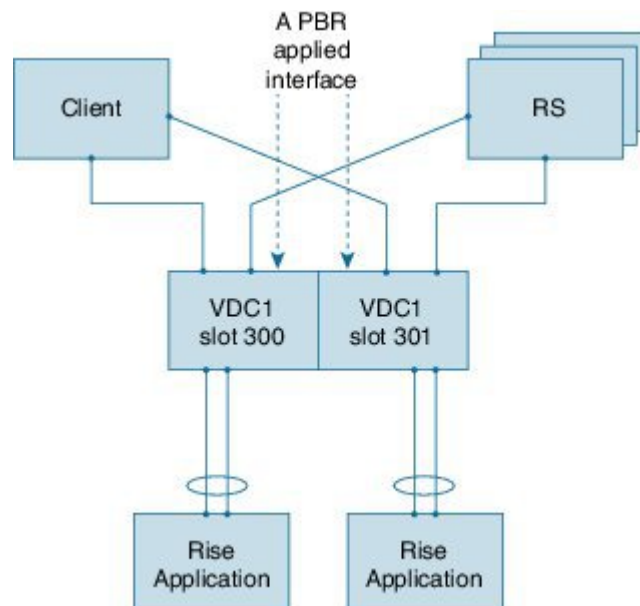
Figure 1: Two Appliances, Two VDCs, One Switch
