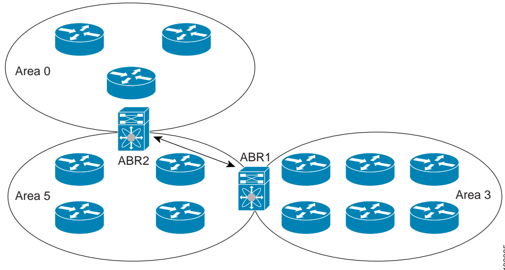
Figure 5-4 Virtual Links
