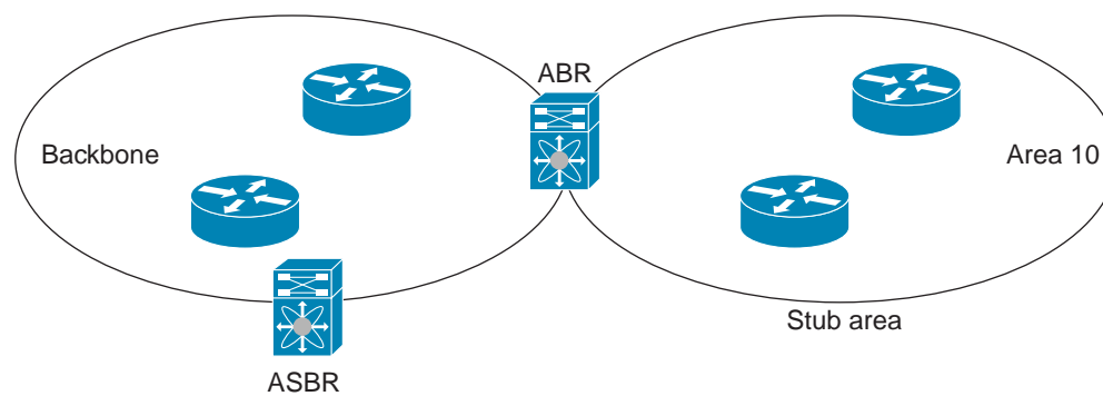
Figure 5-3 Stub Area
