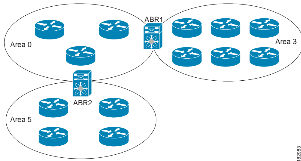
Figure 6-2 OSPFv3 Areas
