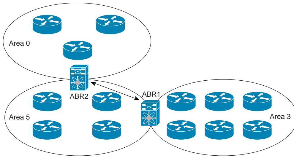
Figure 6-4 Virtual Links
