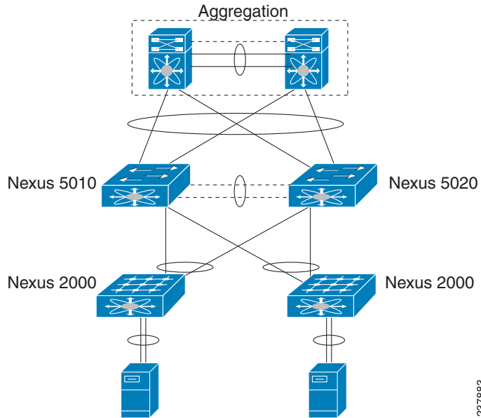
Figure 1-6 vPC-Peered Dual-Supervisor Virtual Modular System Dual-Homed FEXs
