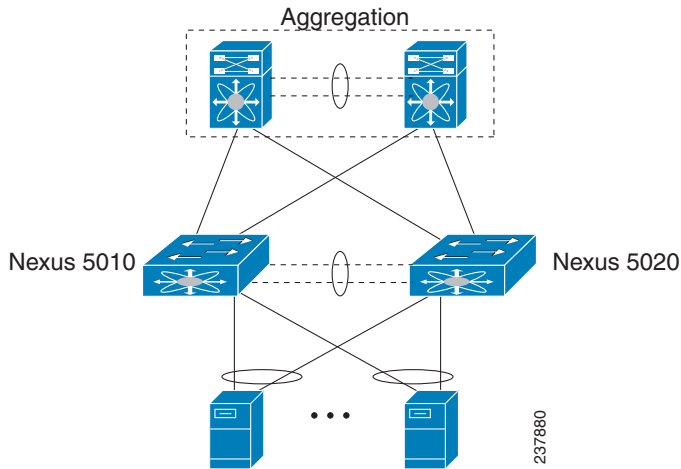
Figure 1-3 vPC Peering Topology
