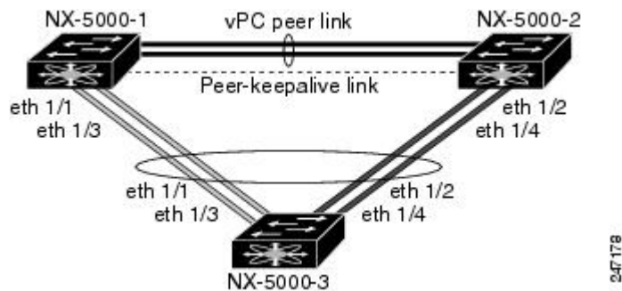
Figure 2: Cisco Nexus 5000 Series Switch-to-Switch vPC Topology
