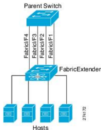
Figure 27: Static Pinning Fabric Interface Connections
