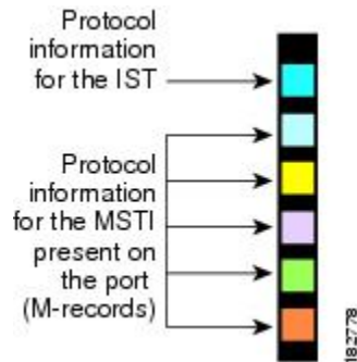
Figure 19: MST BPDU with M-Records for MSTIs
