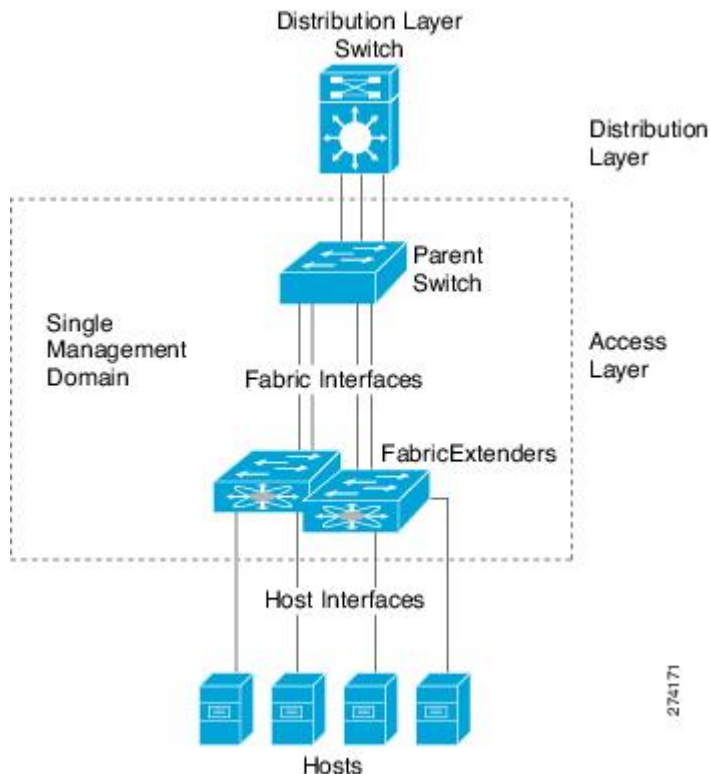
Figure 25: Single Management Domain
