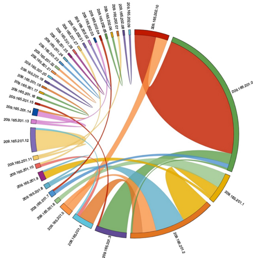
Figure 7: Anomaly Visualization
