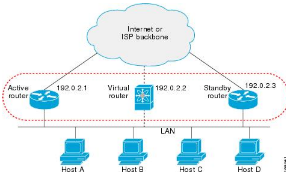
Figure 1: HSRP Topology with Two Enabled Routers
