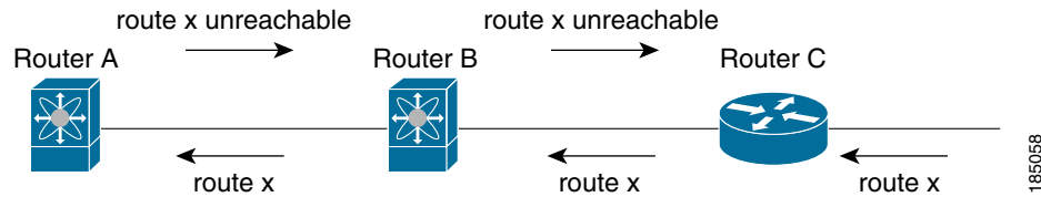
Figure 8-1 RIP with Split Horizon Poison Reverse
