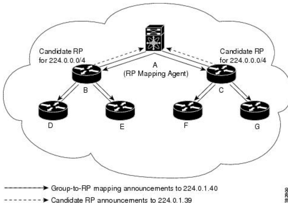
Figure 2: Auto-RP Mechanism
