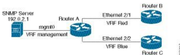
Figure 8: Service VRF Reachability Filtering
