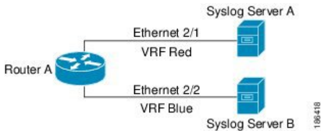
Figure 7: Service VRF Filtering
