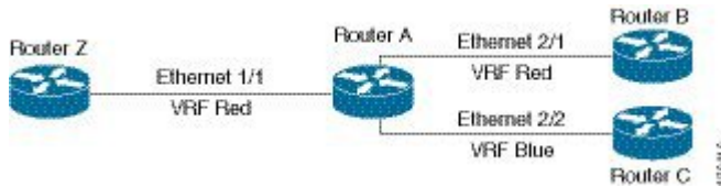
Figure 5: VRFs in a Network
