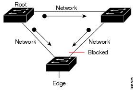
Figure 1: Network with Normal STP Topology
