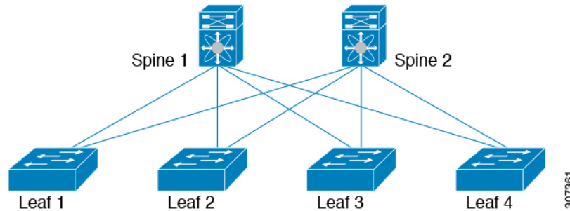
Figure 1: Spine/Leaf Topology
