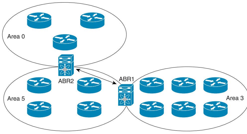
Figure 3-4 Virtual Links
