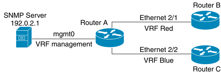
Figure 14-4 Service VRF Reachability Filtering
