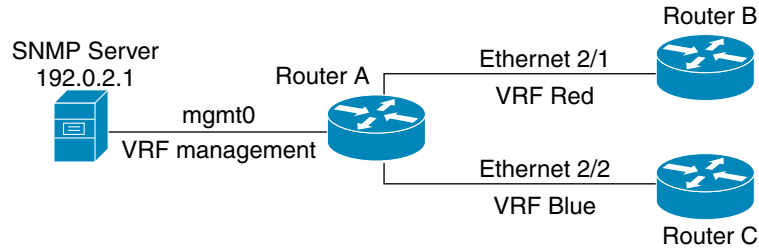
Figure 9-4 Service VRF Reachability Filtering
