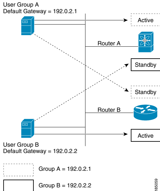
Figure 12-2 HSRP Load Sharing
