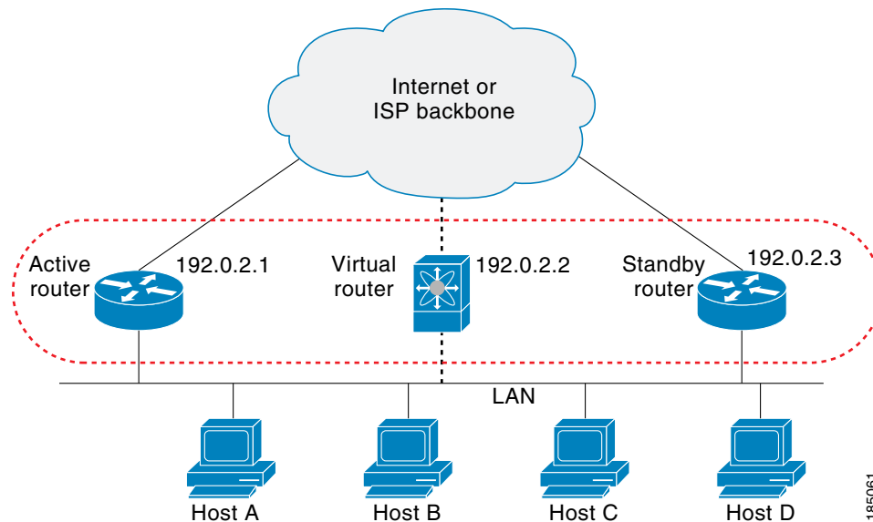
Figure 12-1 HSRP Topology With Two Enabled Routers
