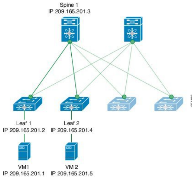
Figure 3: VXLAN Network
