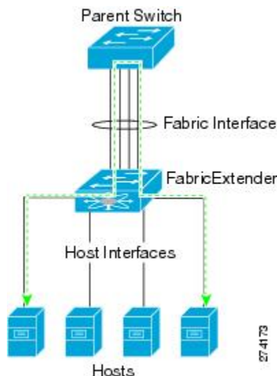
Figure 1: Forwarding Model
