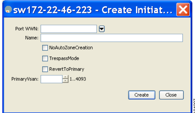
Figure 4-34 Create Initiator Specific Target Dialog Box
