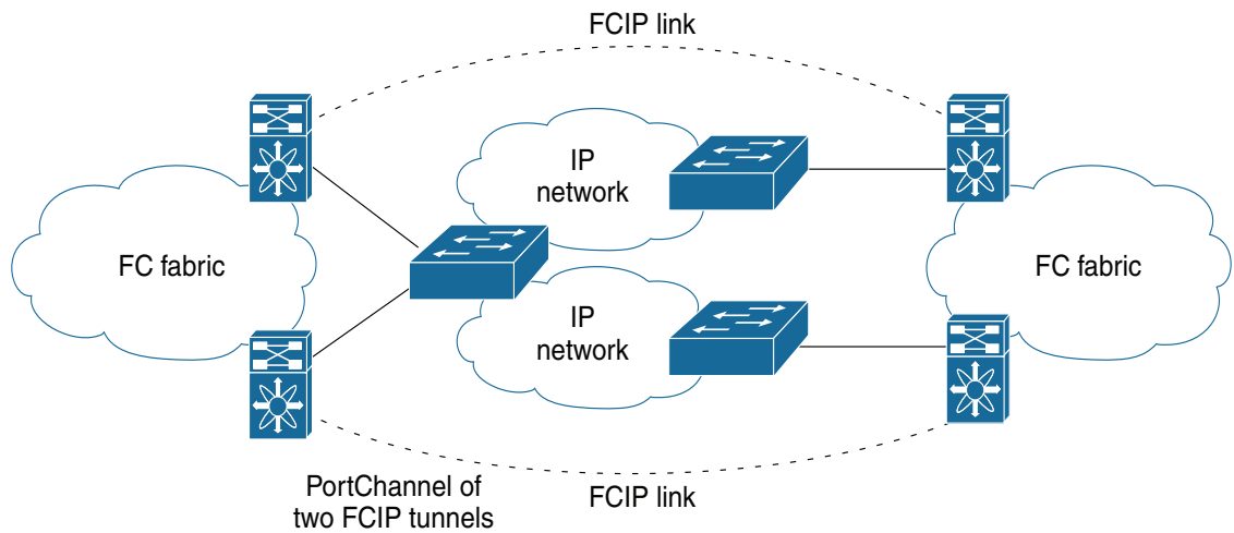
Figure 2-5 FSPF-Based Load Balancing
