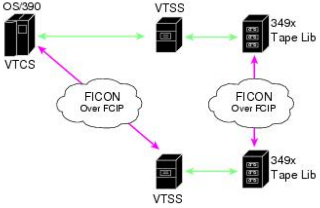
Figure 8: Host Accessing Peer-to-Peer VTS (Virtual Tape Server)
