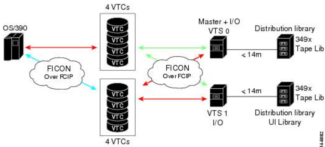
Figure 8: Host Accessing Peer-to-Peer VTS (Virtual Tape Server)
