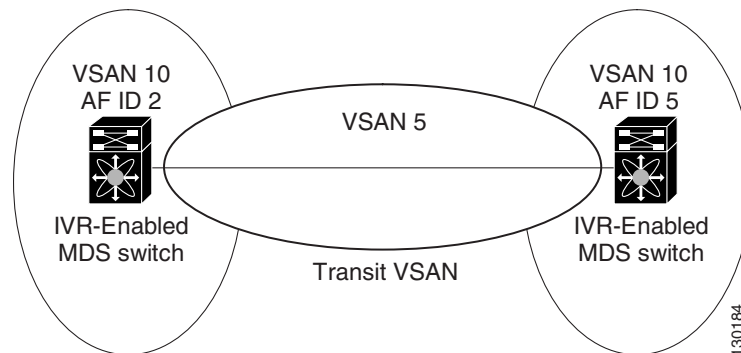
Figure 1-1 Example IVR Topology with Non-Unique VSAN IDs Using AFIDs
