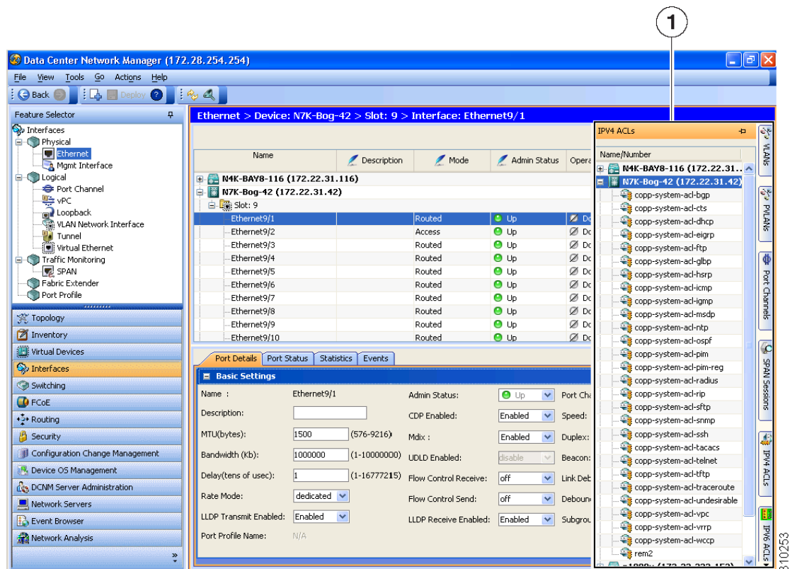
Figure 14-2 Association Pane
