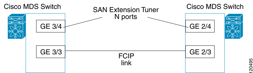
Figure 49-3 Logical Example of N Port Tuning for a FCIP Link
