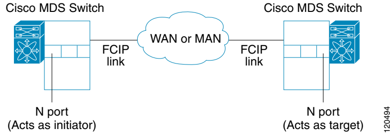
Figure 49-2 N Port Tuning Configuration Physical Example
