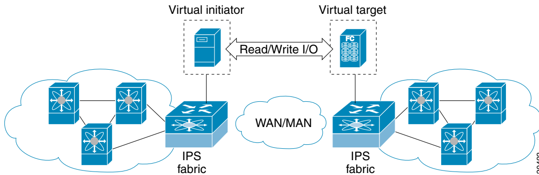
Figure 49-1 SCSI Command Generation to the Virtual Target
