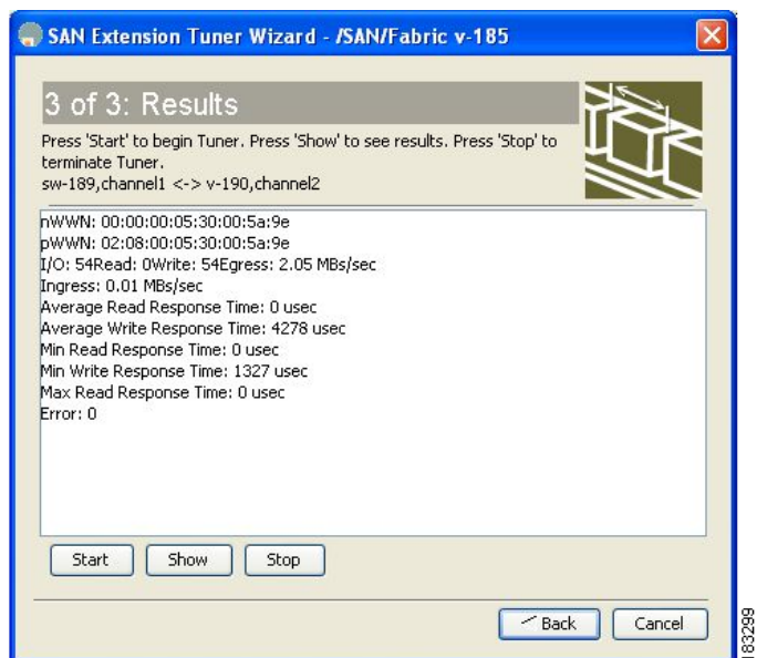
Figure 49-6 Results Dialog Box
