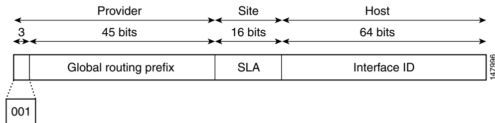
Figure 47-1 Global Address Format
