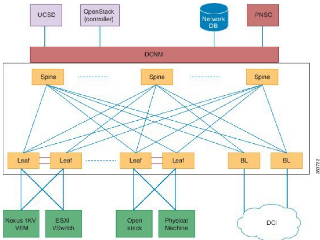
Figure 1: Components in the Cisco DFA Network
