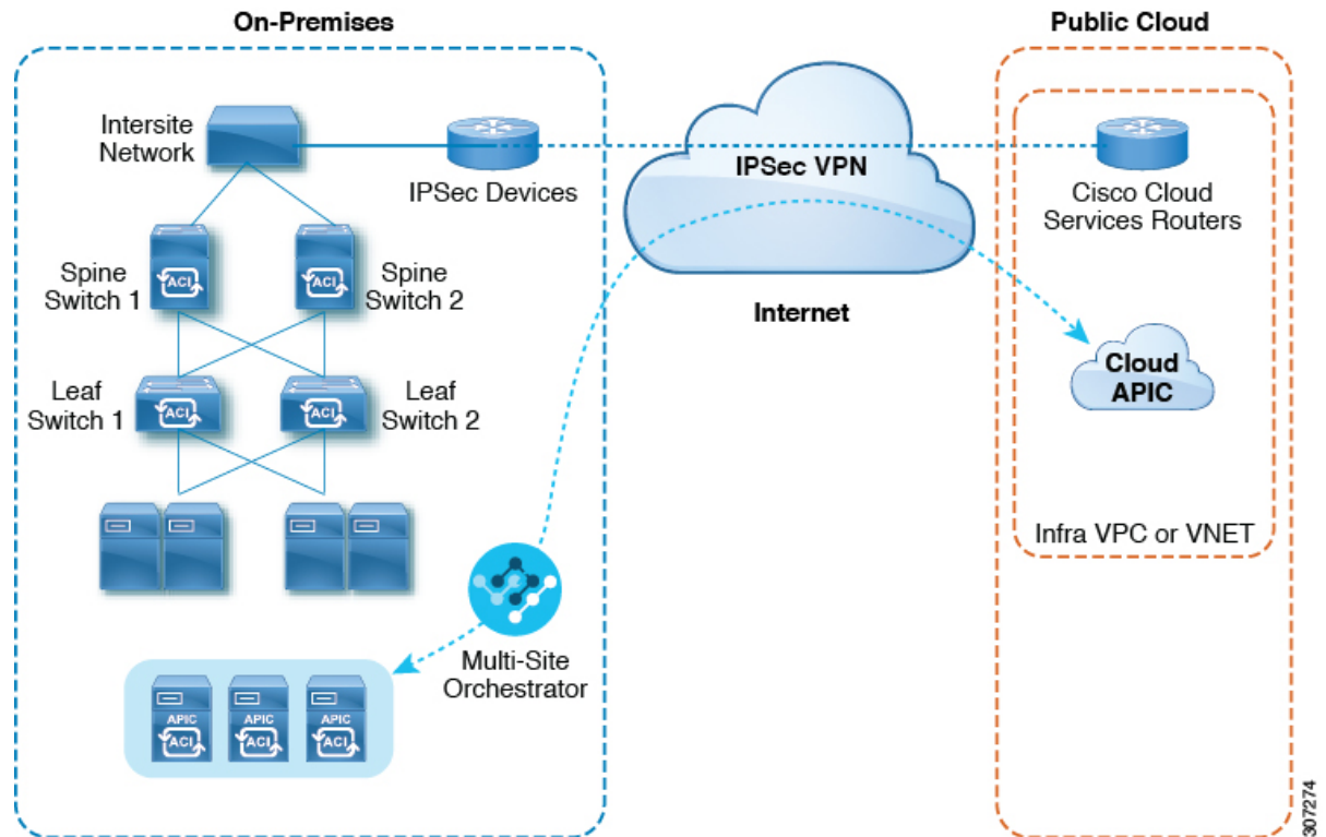
Figure 1: Cisco Cloud APIC Architecture
