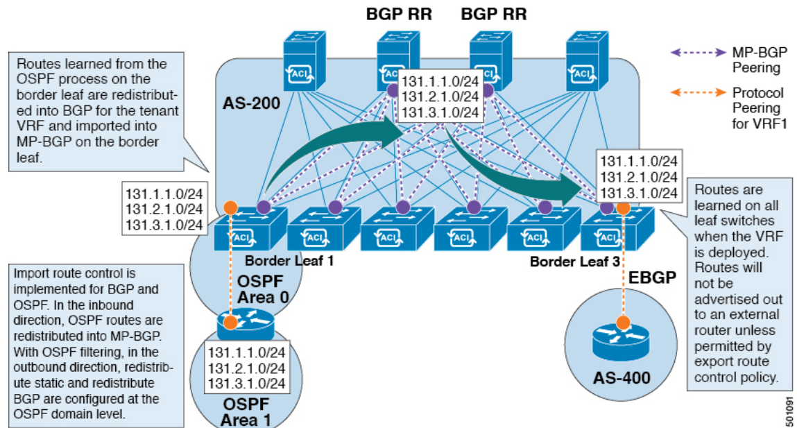
Figure 3: ACI Route Redistribution
