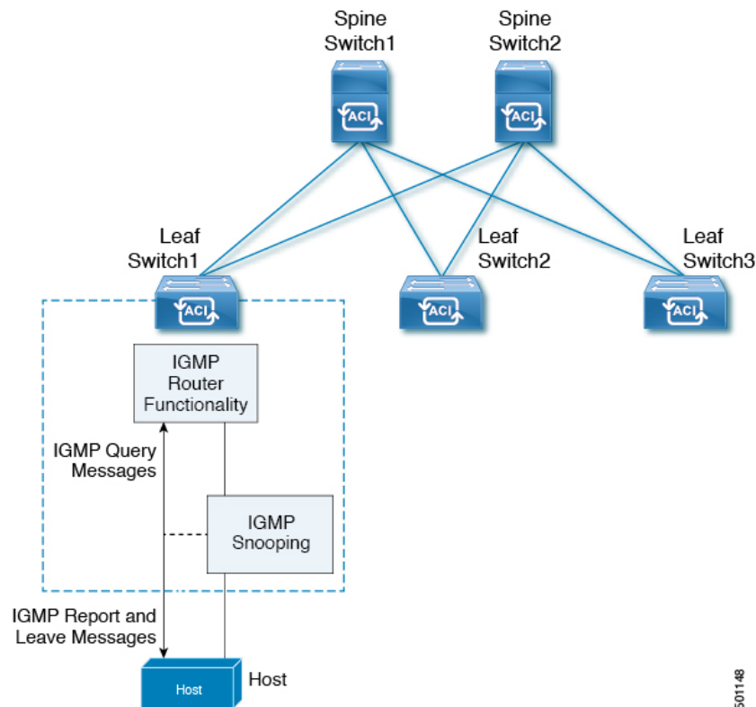
Figure 14: IGMP Snooping function
