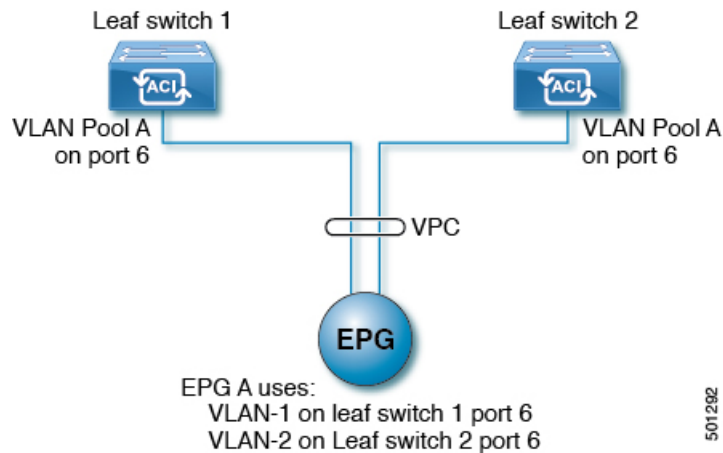
Figure 9: VLANs for Two Legs of a vPC
