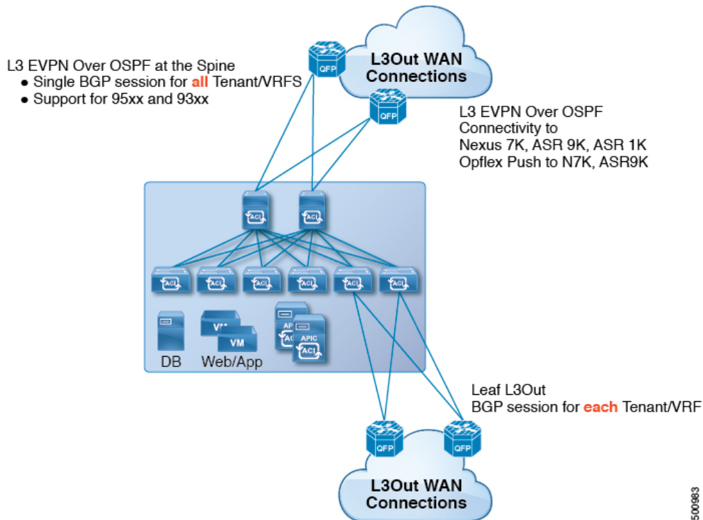
Figure 18: Cisco ACI GOLF Topology
