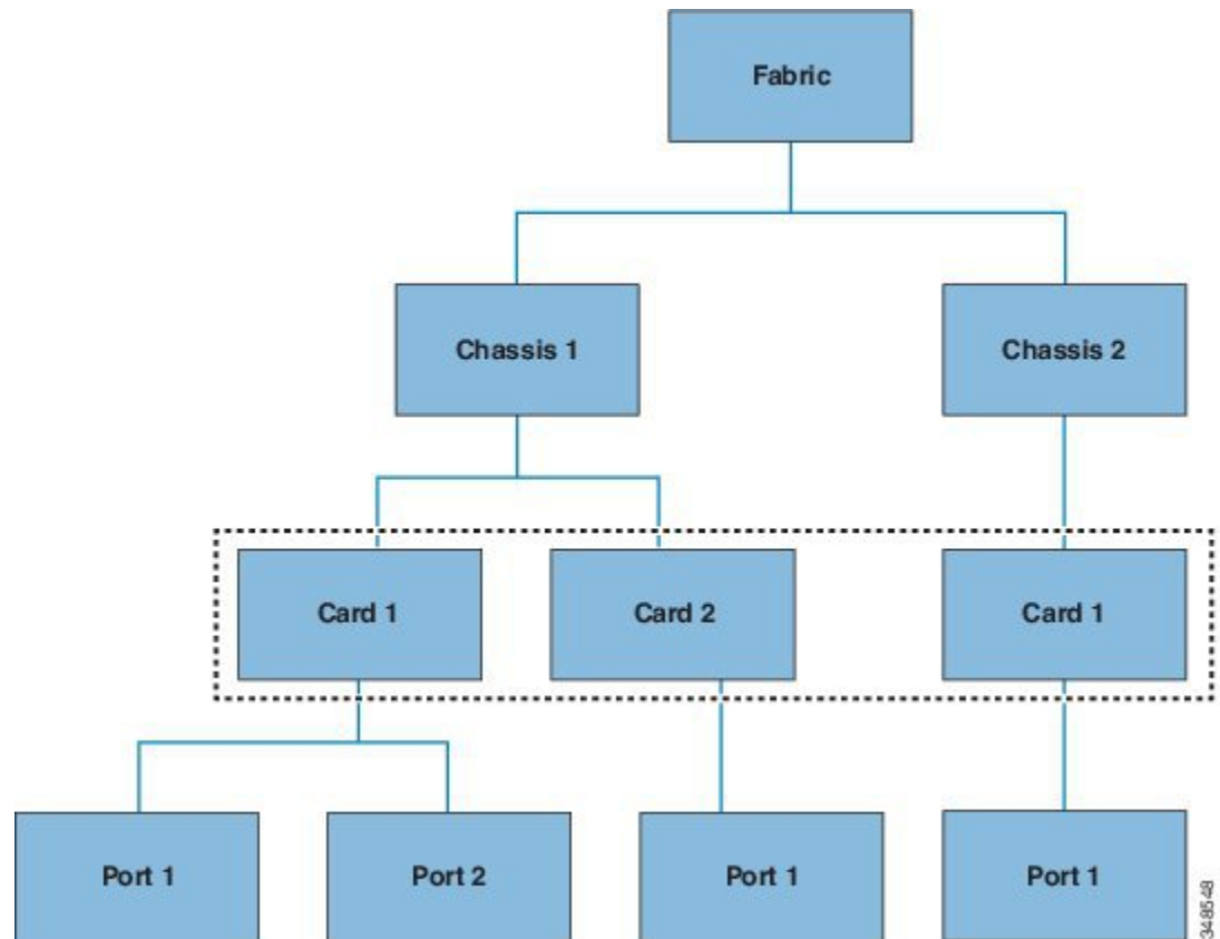
Figure 7: Class-Level Queries
