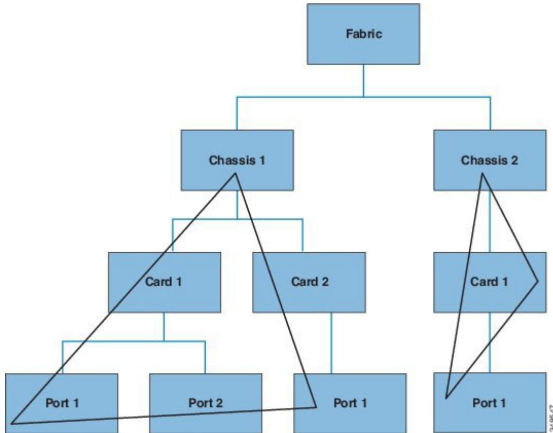
Figure 6: Tree-Level Queries
