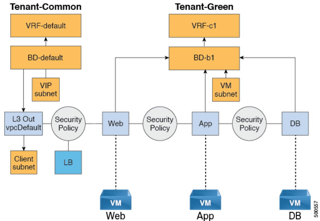
Figure 13: VPC Plan - Load Balancer Only
