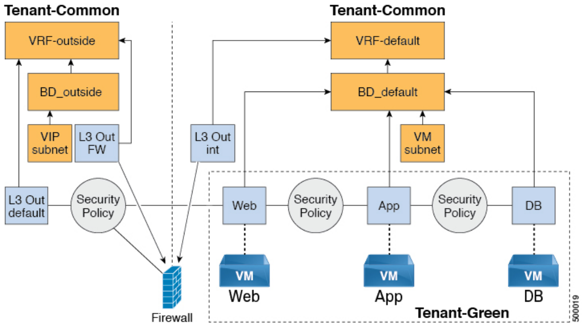
Figure 14: Shared Plan - Perimeter Firewall Only Overview
