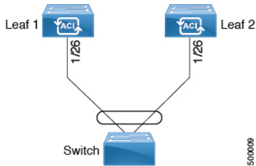
Figure 5: Virtual port channel configuration
