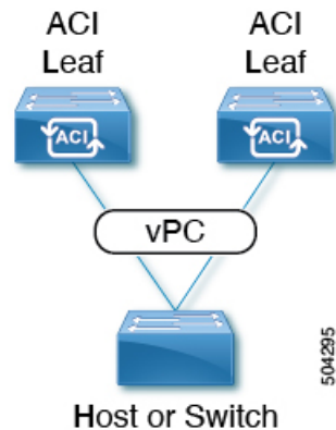
Figure 4: vPC Domain
