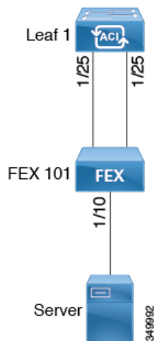
Figure 11: Basic FEX Configuration
