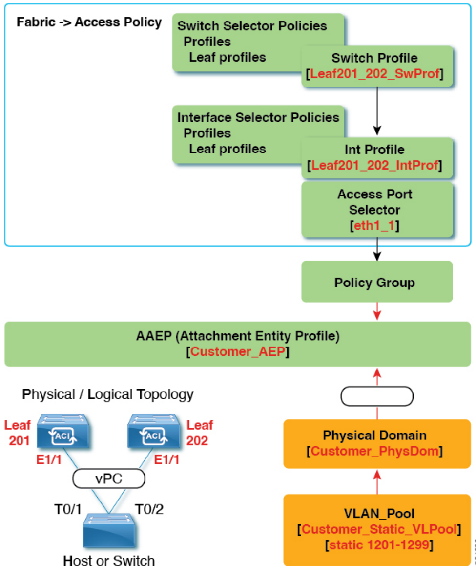
Figure 6: vPC With the Same Leaf Switch Interfaces Across Two Leaf Switches With Combined Profiles
