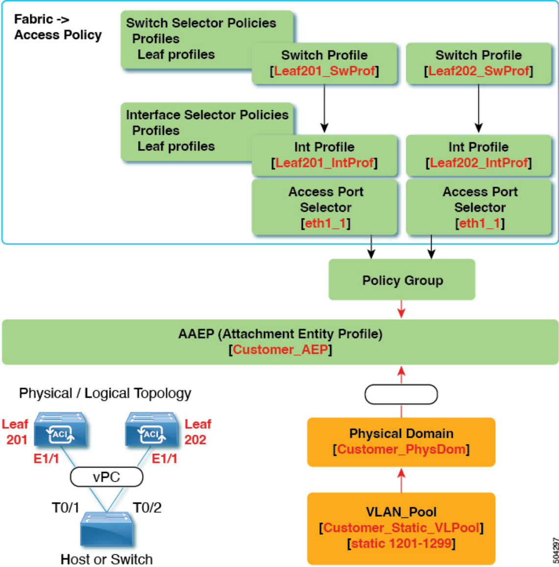
Figure 7: vPC With the Same Leaf Switch Interfaces Across Two Leaf Switches with Individual Profiles
