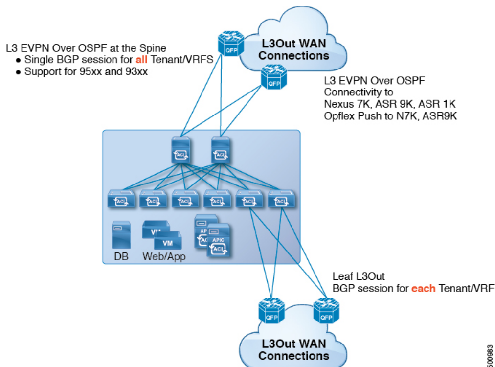
Figure 18: Cisco ACI GOLF Topology
