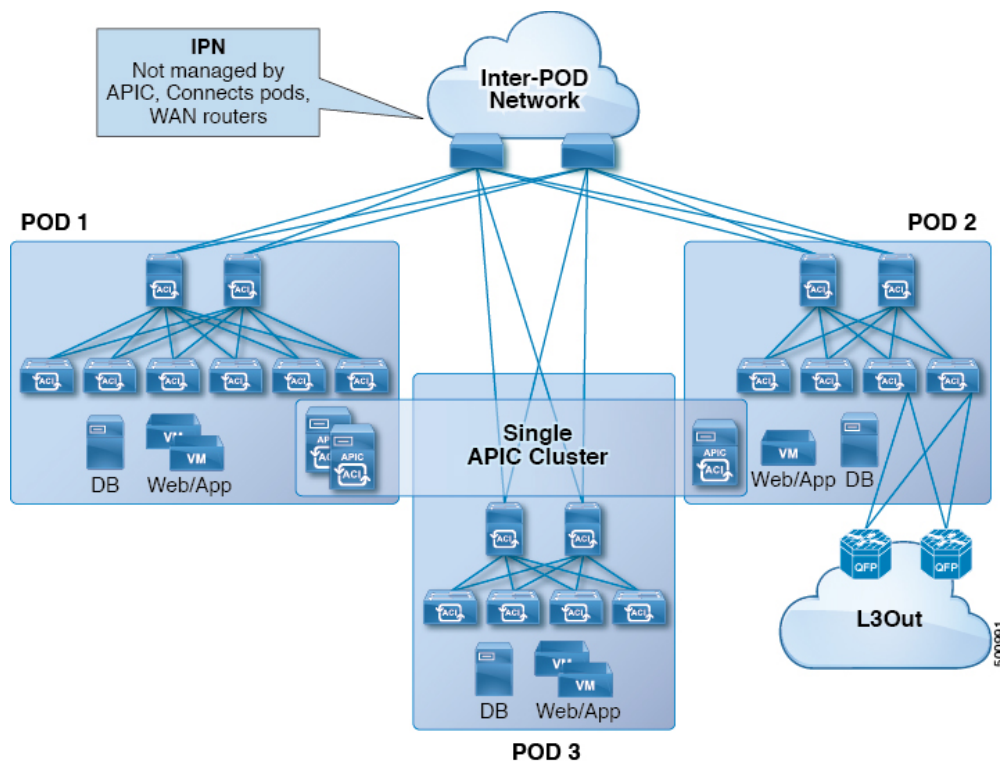
Figure 19: Multipod Overview
