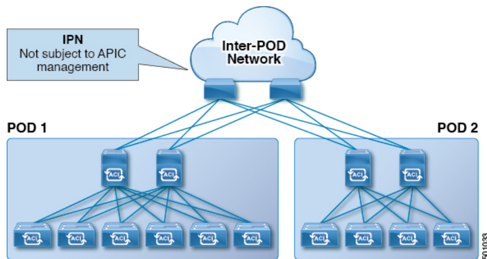
Figure 21: Multipod Topology
