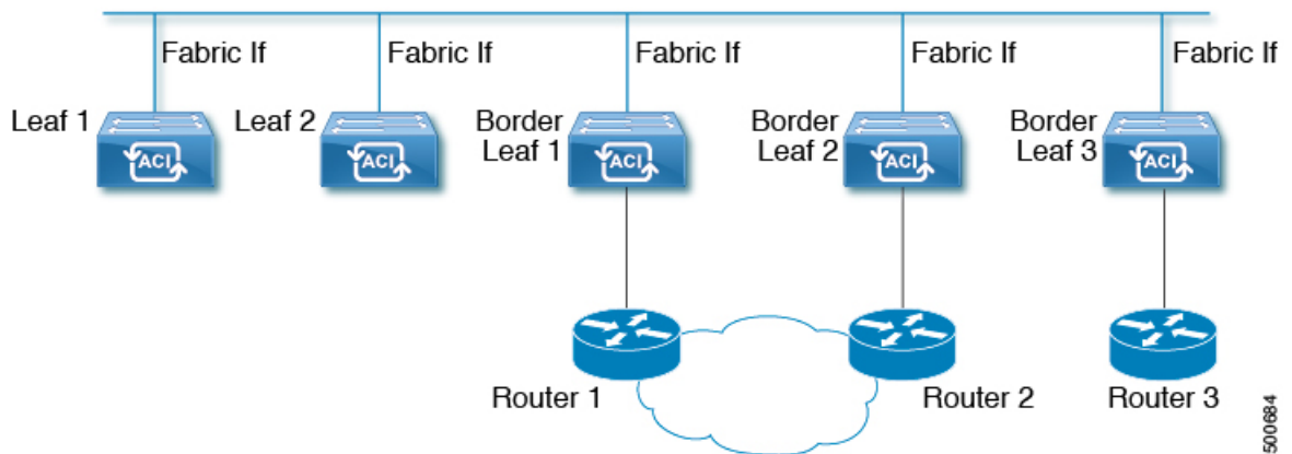
Figure 17: Fabric for Multicast routing
