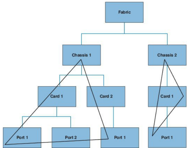
Figure 6: Tree-Level Queries
