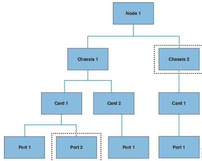
Figure 8: Object-Level Queries
