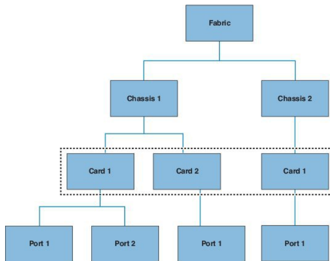
Figure 7: Class-Level Queries
