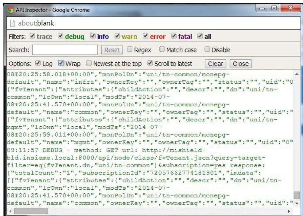
Figure 2: API Inspector
