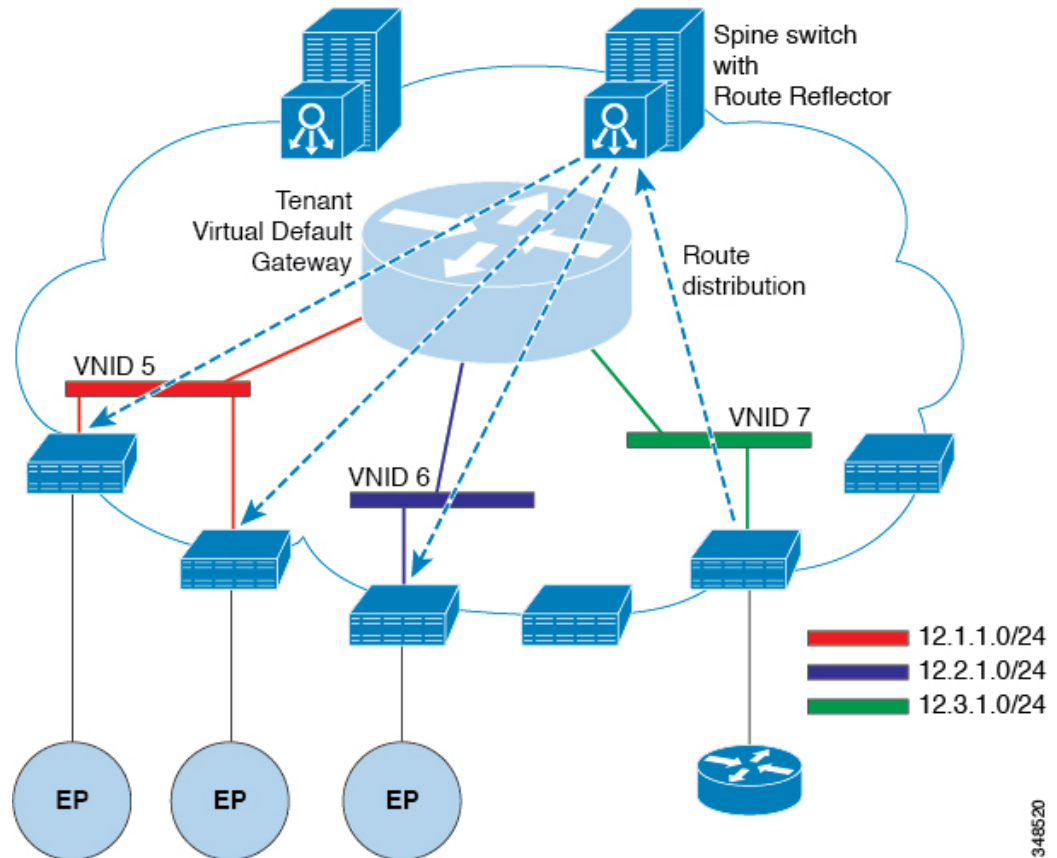
Figure 1: Router Peering
