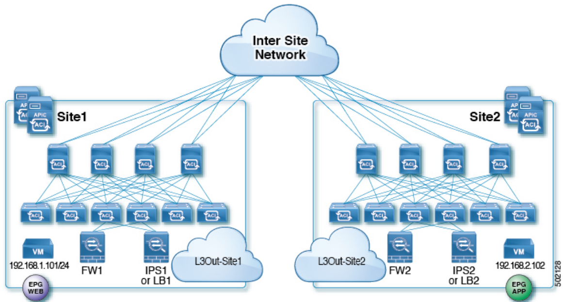
Figure 1: Cisco ACI Multi-Site Service Integration Topology
