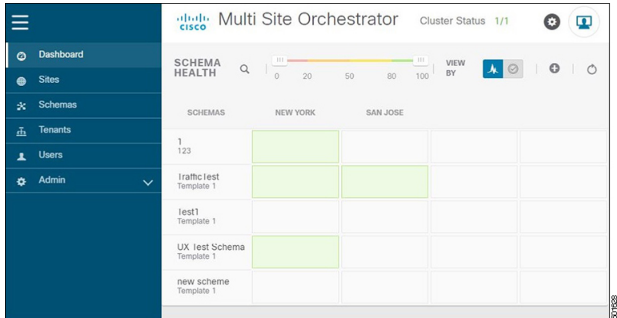
Figure 1: Multi-Site Dashboard
