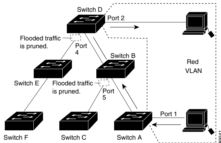
Figure 5-2 Optimized Flooded Traffic with VTP Pruning
