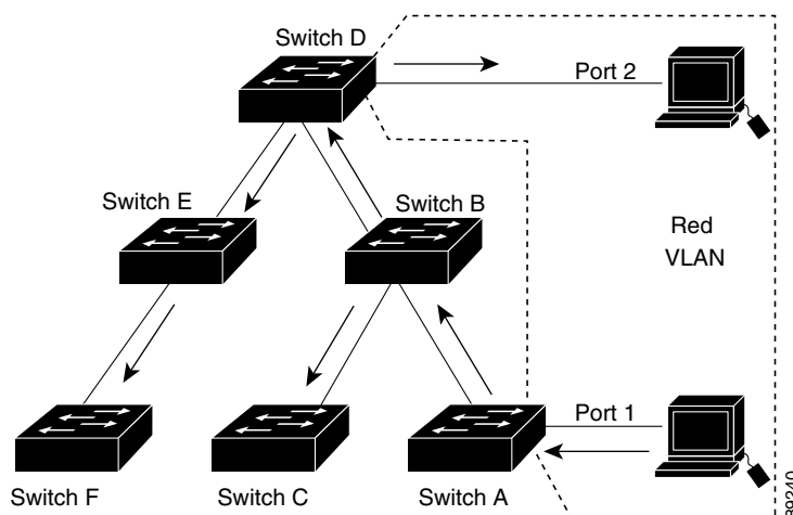
Figure 5-1 Flooding Traffic without VTP Pruning
