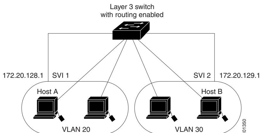
Figure 6 Connecting VLANs with the Switch
