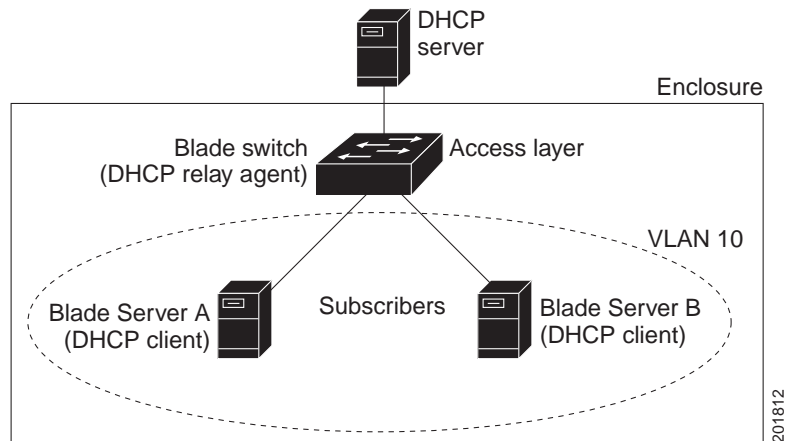
Figure 21-1 DHCP Relay Agent in a Metropolitan Ethernet Network
