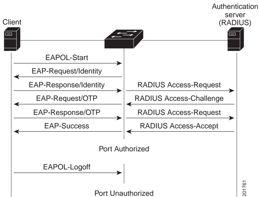
Figure 9-3 Message Exchange
