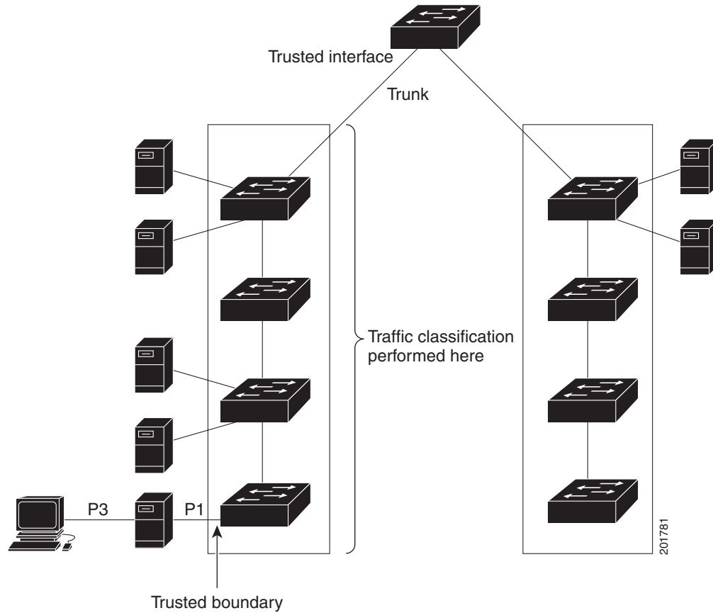
Figure 36-12 Port Trusted States within the QoS Domain
