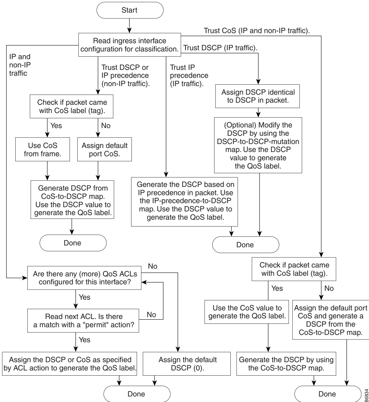
Figure 36-3 Classification Flowchart
