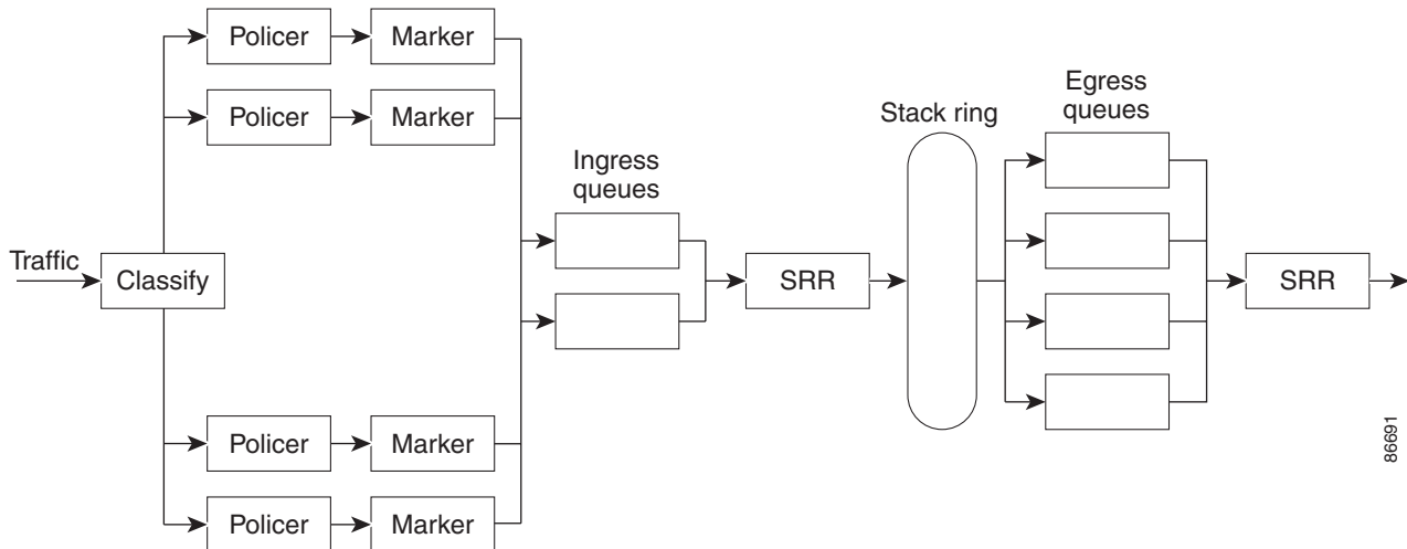
Figure 36-6 Ingress and Egress Queue Location
