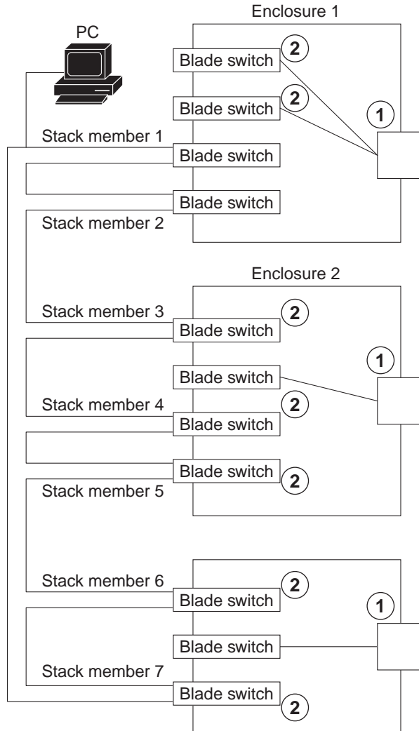
Figure 10-3 Connecting a Switch Stack to a PC
