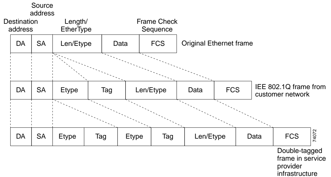
Figure 15-2 Original (Normal), IEEE 802.1Q, and Double-Tagged Ethernet Packet Formats
