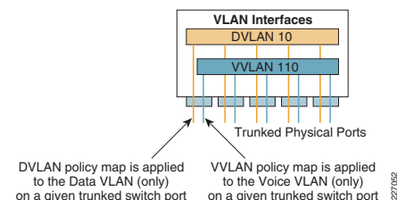
Figure 4 Per-Port/Per-VLAN-Based QoS
