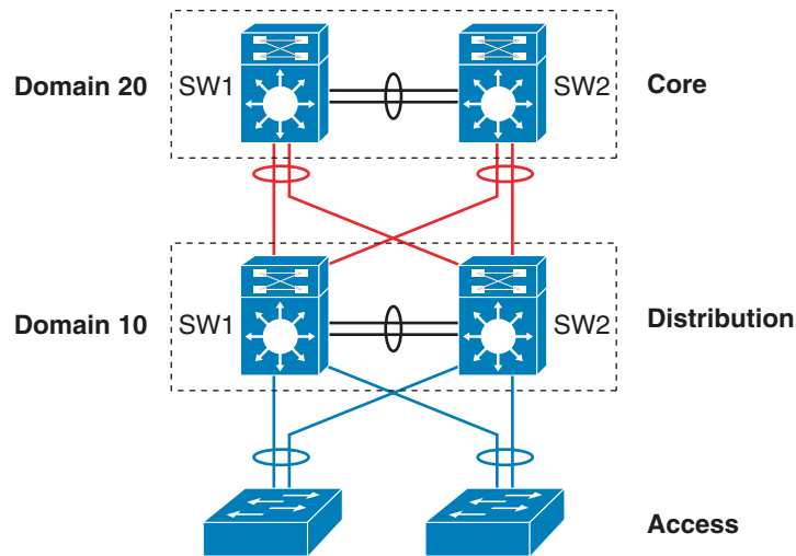
Figure 3-25 VSS Domain and Switch ID
