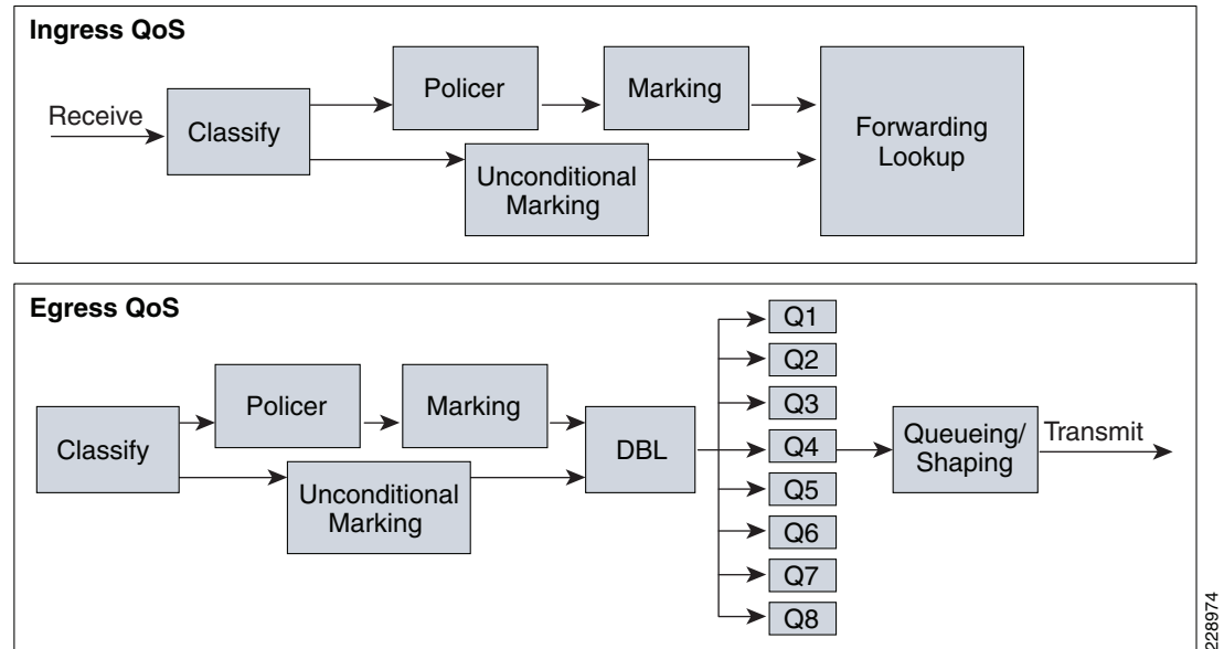
Figure 3-50 Catalyst 4500 - Supervisor 6-E and 6L-E QoS Architecture
