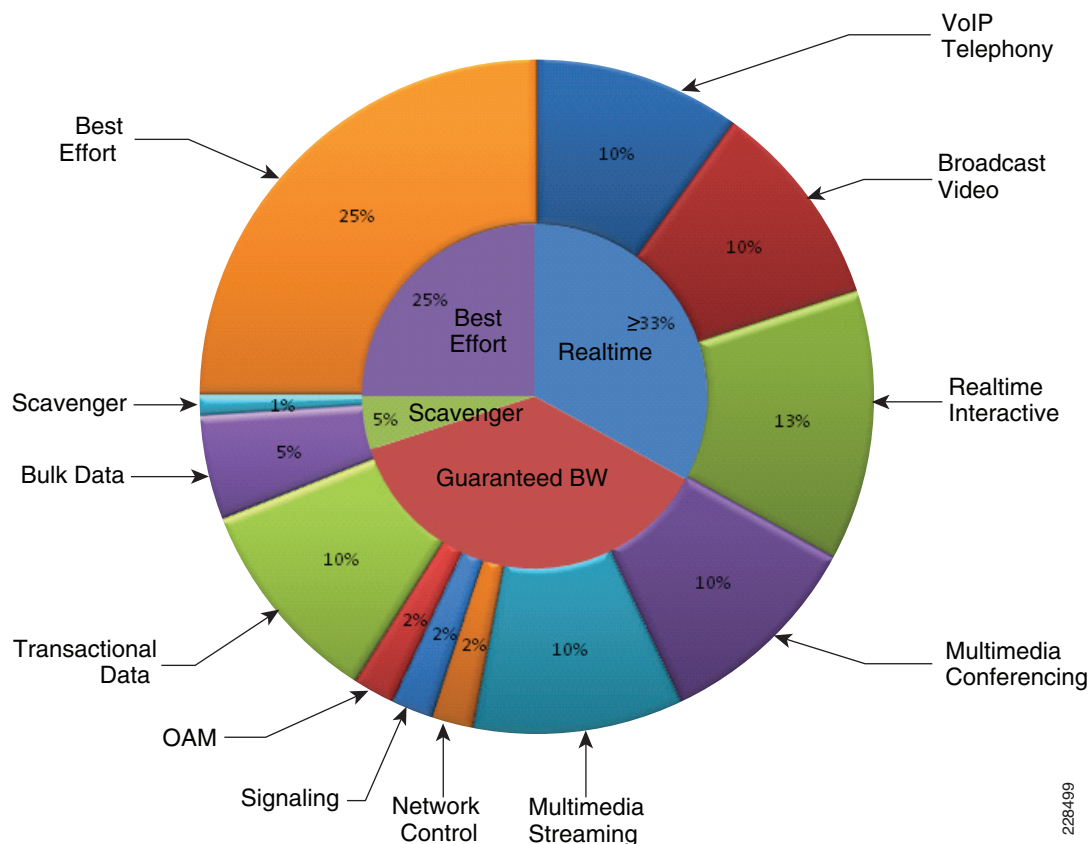
Figure 3-48 Compatible 4-Class and 12-Class Queuing Models
